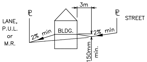
FRONT TO BACK DRAINAGE
