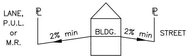
SPLIT DRAINAGE
